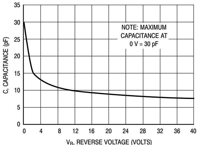
Figure 6. Maximum Capacitance
